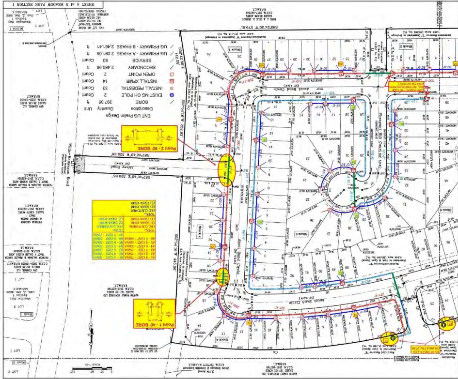
Appendix 4G: IMPROVEMENT AREA 1 MAP, SECTION 1: PROPOSED ELECTRICAL LAYOUT
