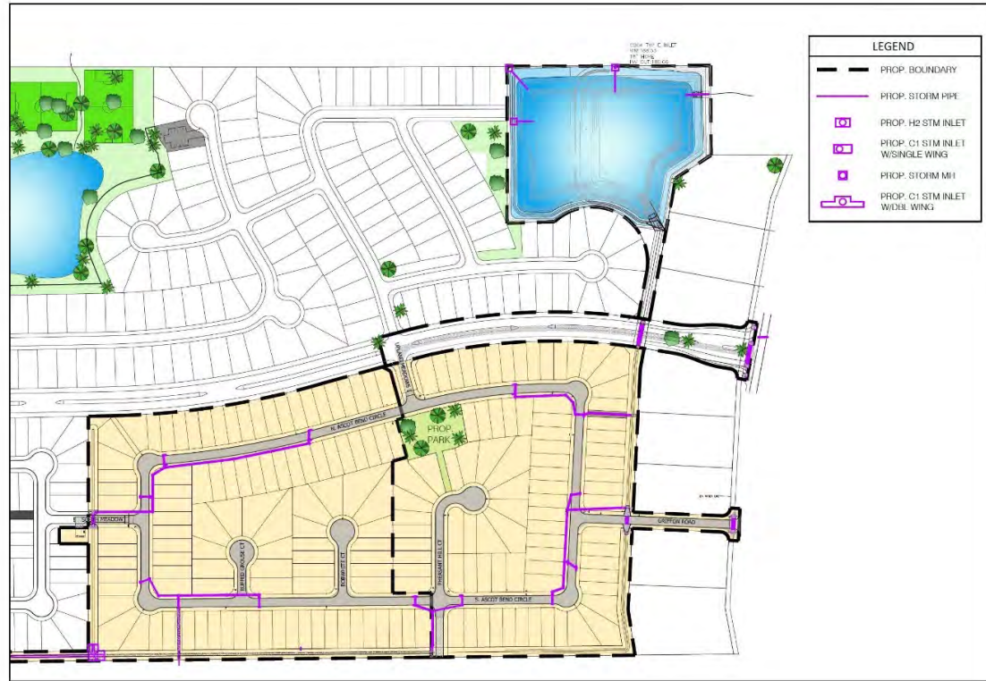
Appendix 4B: IMPROVEMENT AREA 1 MAP: PROPOSED STORM SEWER
