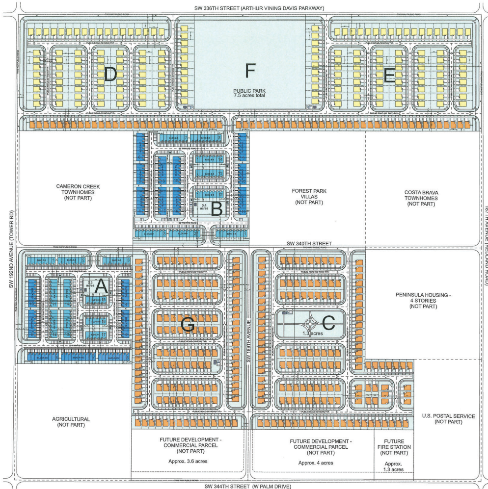
1 MASTER SITE PLAN SCALE: 1" = 100'
